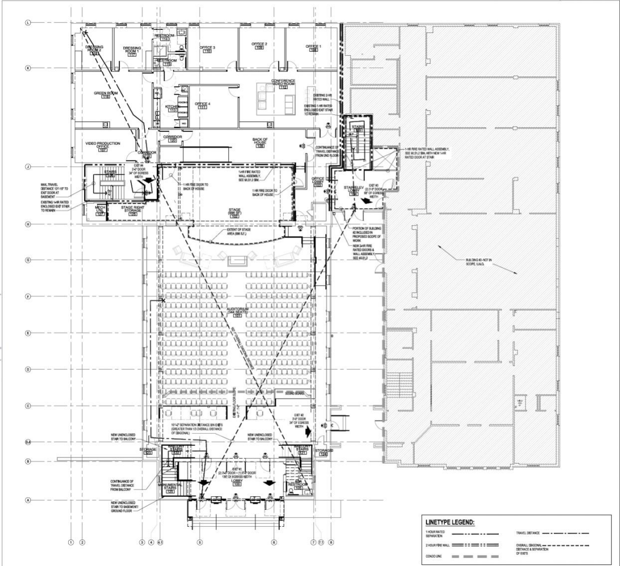
1 FLOOR PLAN (2ND FLOOR) SCALE: 1/8" = 1'-0"
