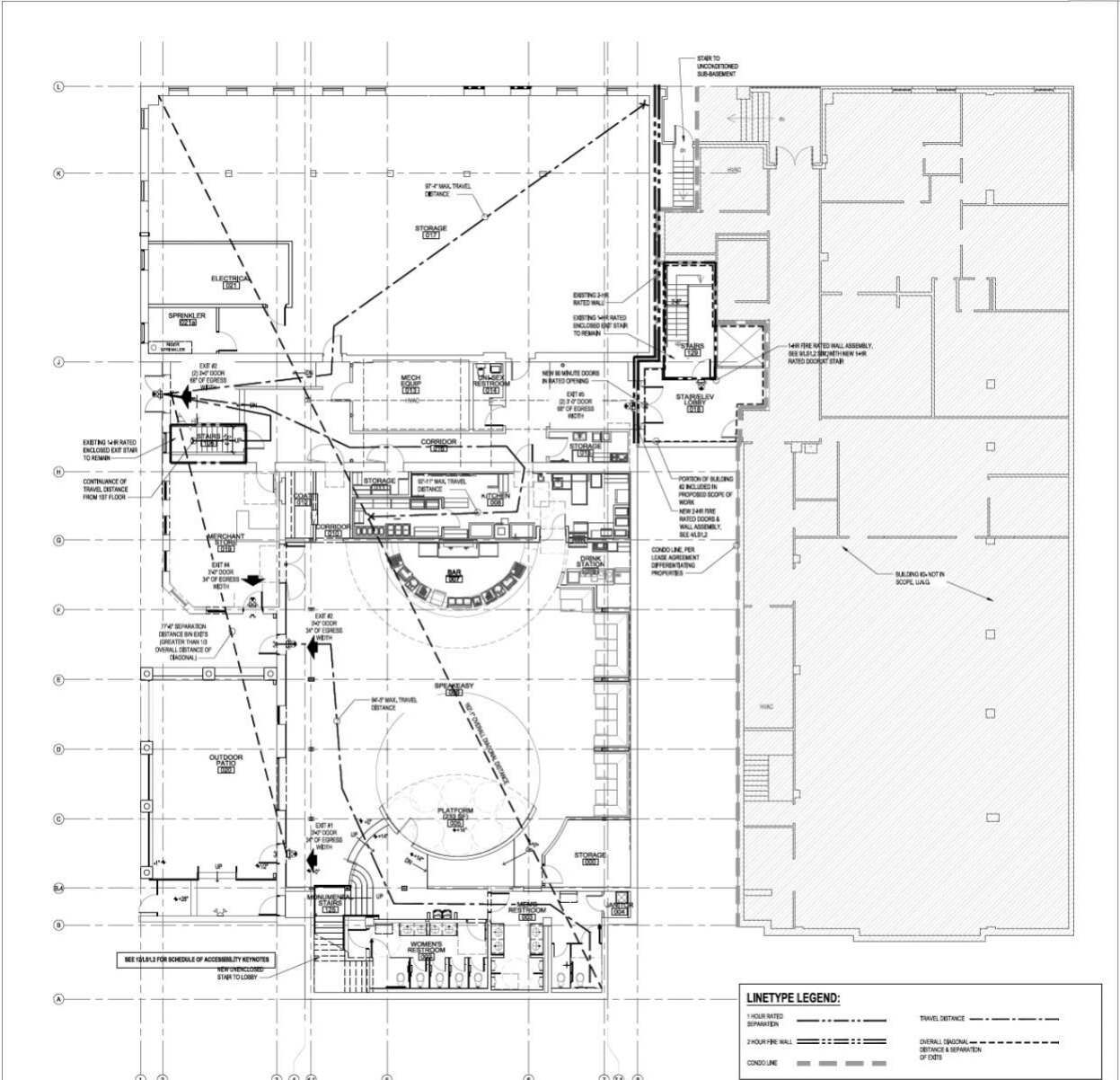
1 LIFE SAFETY PLAN (1ST FLOOR) SCALE: 1/8" = 1'-0"
